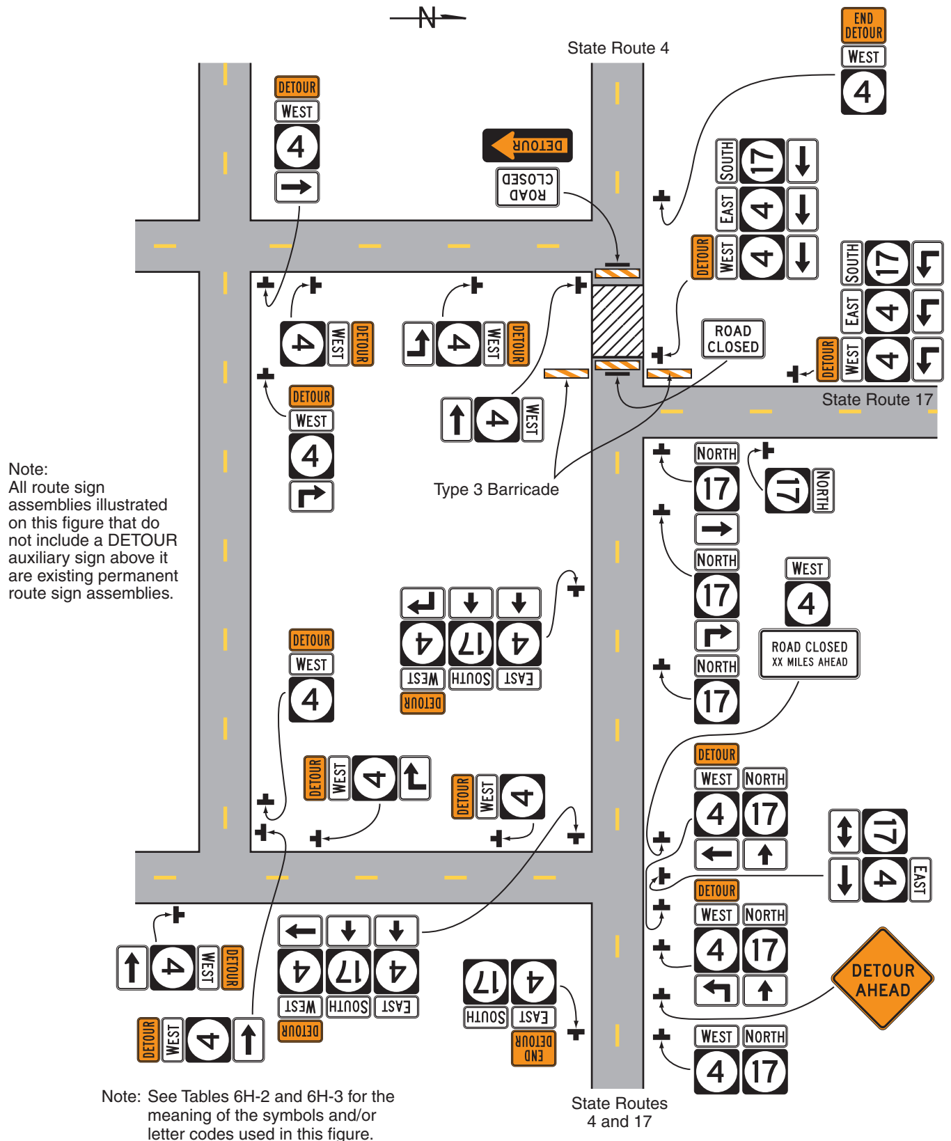
Figure 6H-9. Overlapping Routes with a Detour (TA-9)
