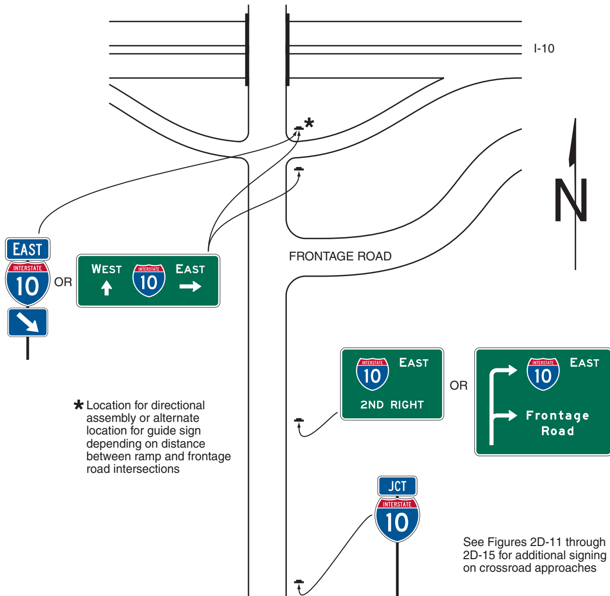
Figure 2D-16. Example of Crossroad Signing for an Entrance Ramp with a Nearby Frontage Road
