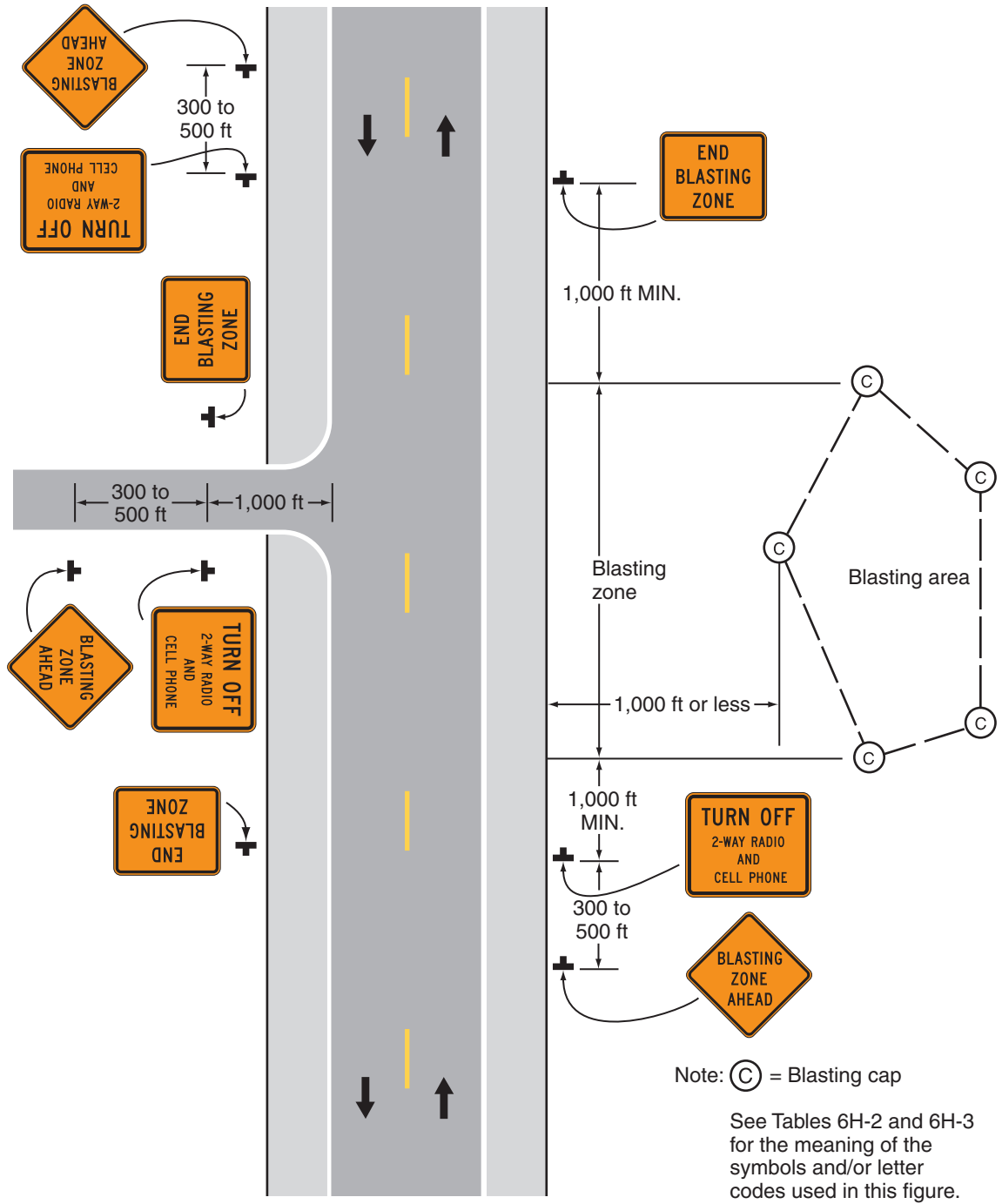
Typical Application 2
