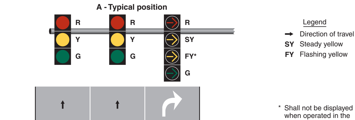
Figure 4D-19. Typical Position and Arrangements of Separate Signal Faces with Flashing Yellow Arrow for Protected/Permissive Mode and Protected Only Mode Right Turns
