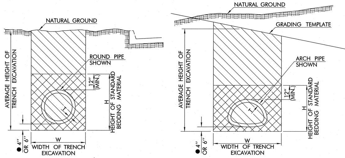
TRENCH EXCAVATION IN CUT SECTIONS
