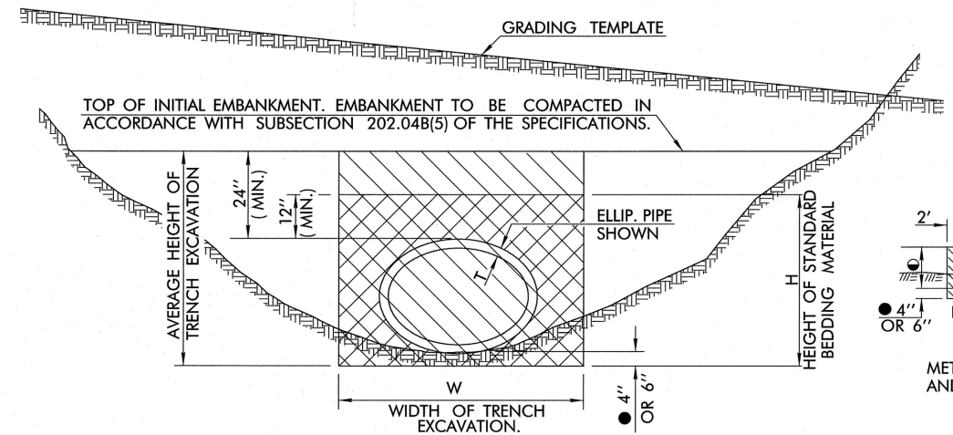
METHOD NO. 1 TRENCH EXCAVATION IN EMBANKMENT SECTIONS
