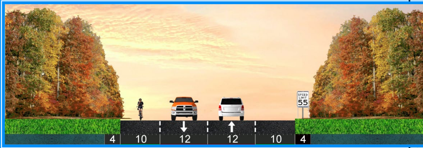
TWO LANE SECTION
