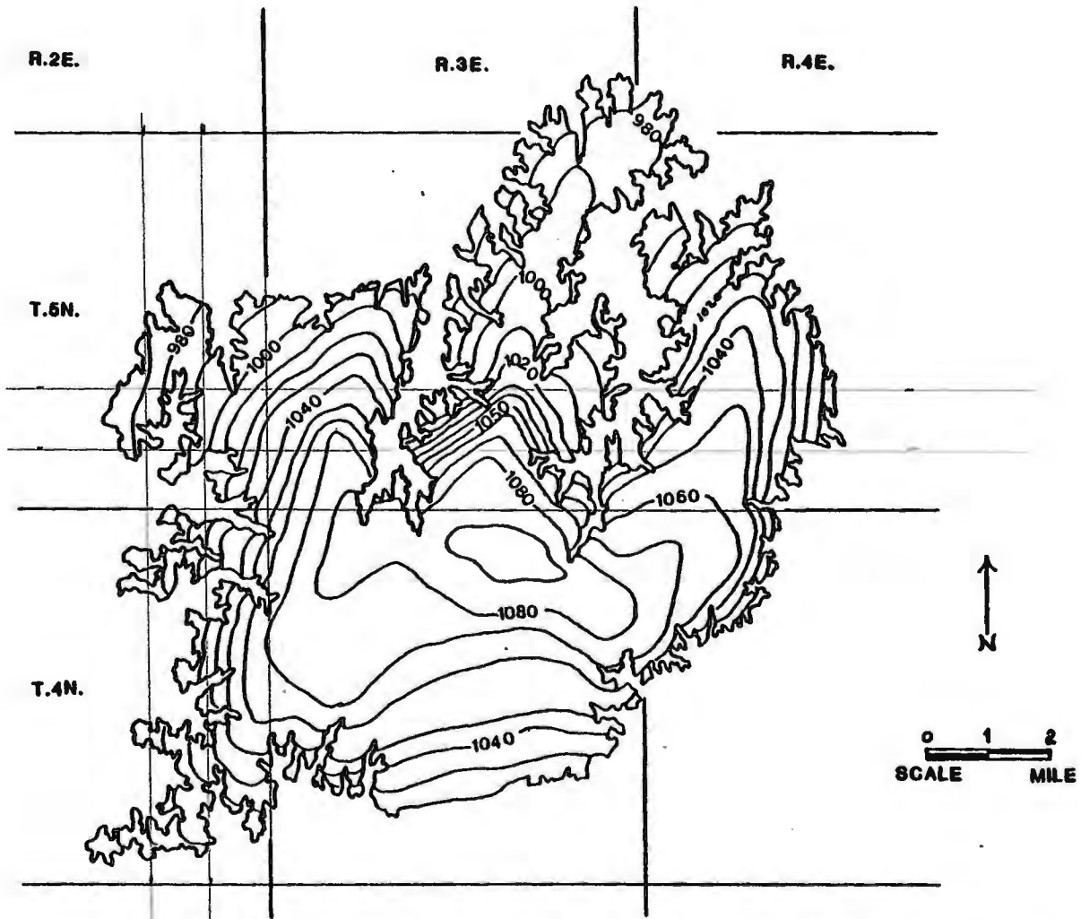
Figure 10. ISOLATED TERRACE DEPOSIT OF THE CANADIAN RIVER OF GARVIN, McCLAIN, AND PONTOTOC COUNTIES, OKLAHOMA. AUGUST 12, 13, AND 17, 1986 WATER TABLE MAP.
